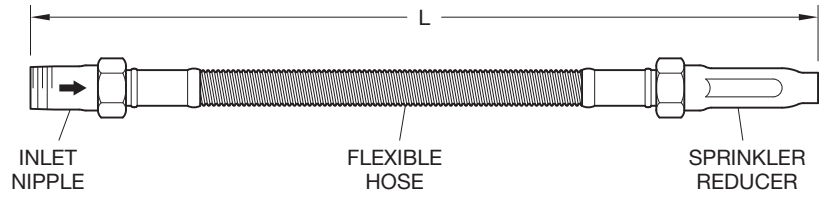
FIGURE 1 MODEL FH-1 FLEXIBLE HOSE NOMINAL DIMENSIONS
